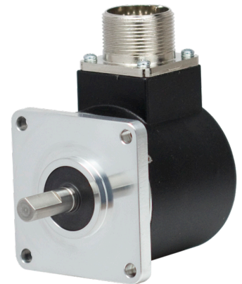
The Model 25SP A Programmable Size 25 Shaft Encoder Comes standard with dual bearings rated 80lbs axial or radial
